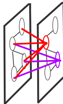
Figure 7: Laplacian smoothing: averaging the neighbourhood information
