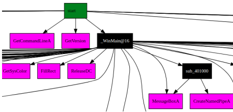
GenCallGdl: call graph without instructions
